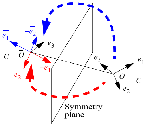
Figure 2. How to relate the virtual view and the real camera's view from the virtual viewpoint.
