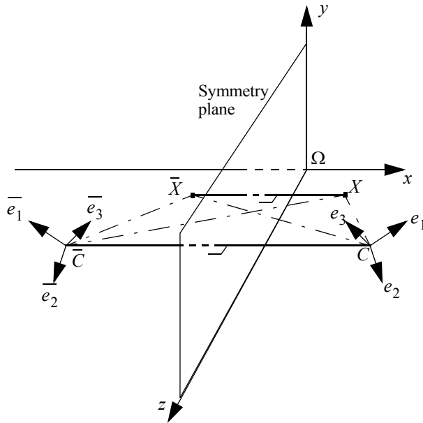
Figure 1. Symmetrical points seen from symmetrical cameras
